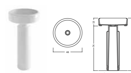
Lavabo freestanding Ø48x87H cm - Freestanding washbasin - Lavabo autoportante
