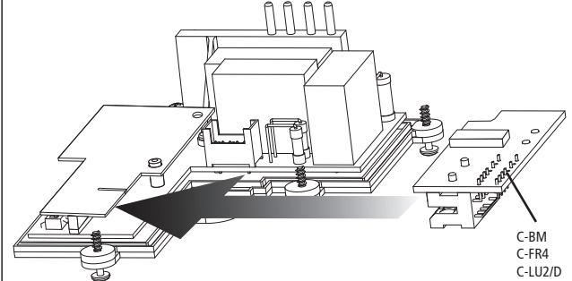
Fig.8-B LIMODOR F/M-EC
