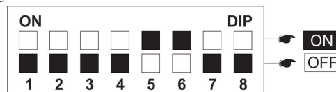
DIP-Switch C-NR
